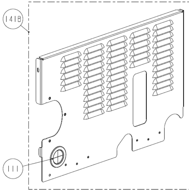
VENCLOSURE REAR PANEL (REARX)
